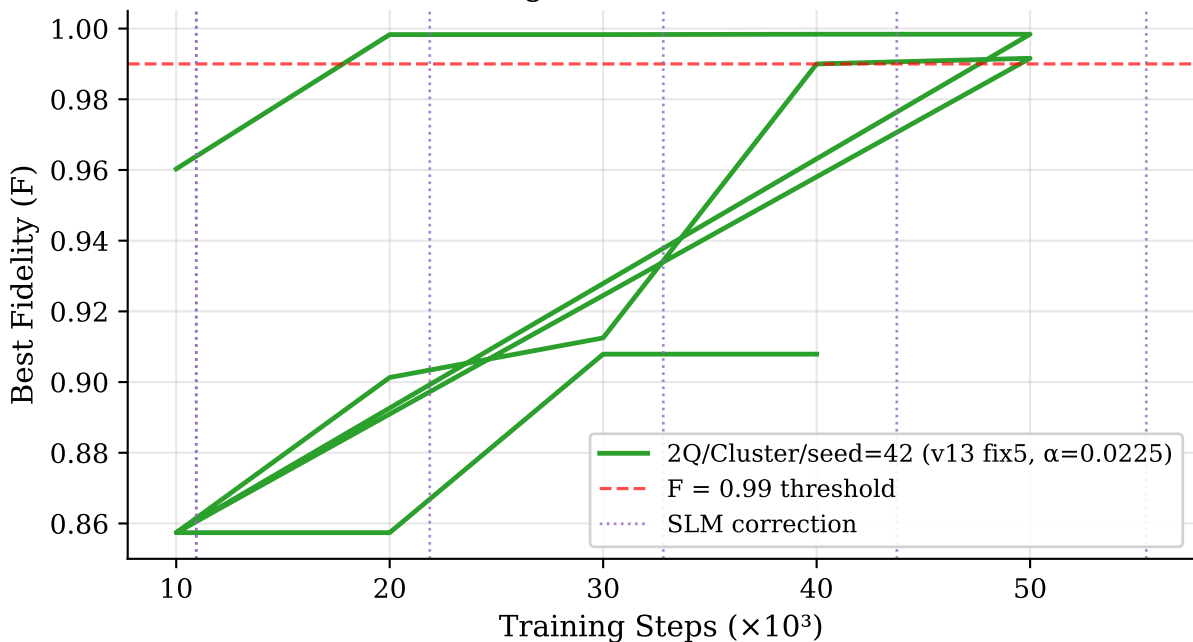
QUASAR v13: Fidelity vs Training Steps (Cluster-linear Target, 2 Qubits, DEHB Search Phase)
