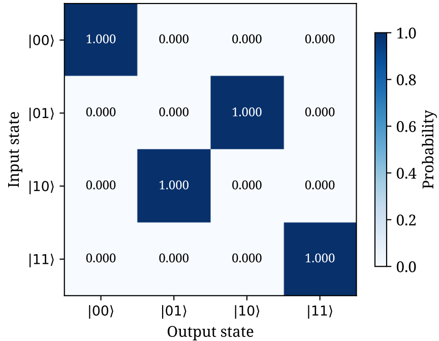
(c) Encoded SWAP Verification
