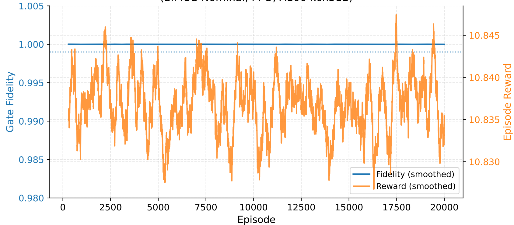
TensorBoard-Style Training Monitor — R3 Seed 0 (SiMOS Nominal, PPO, A100 kcn512)
