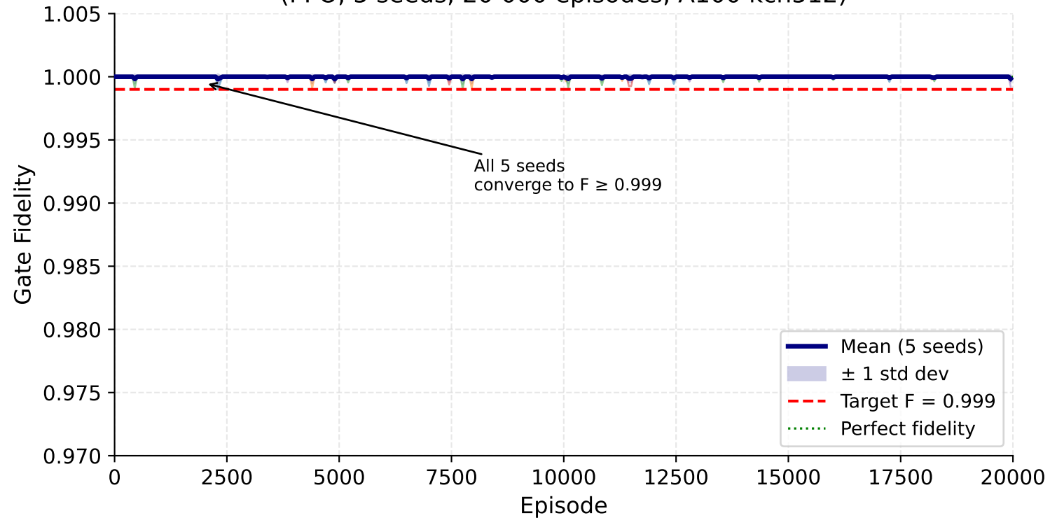
Fidelity vs Episode — R3 SiMOS Nominal (PPO, 5 seeds, 20 000 episodes, A100 kcn512)
