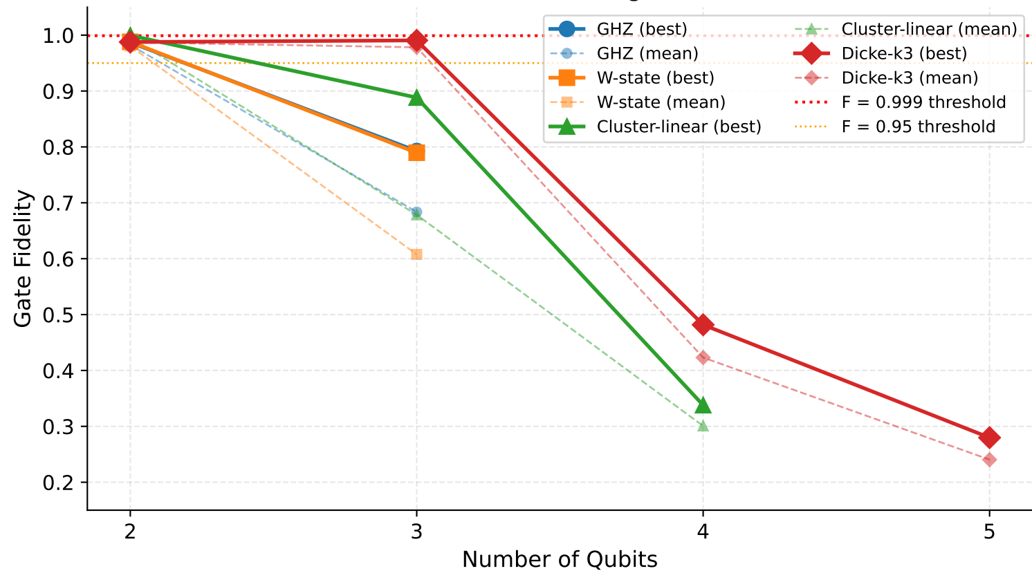
Scaling Ablation — Fidelity vs Qubit Count (SiliQun + PPO, all 4 target families)
