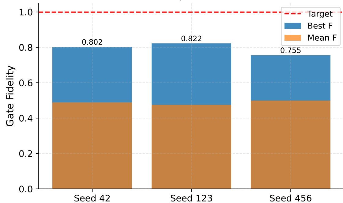
R1 — Daraeizadeh Replication (PPO, 10 000 episodes, SiMOS CZ)
