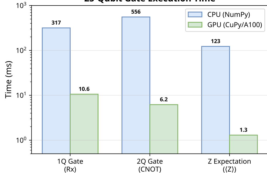
25-Qubit Gate Execution Time
