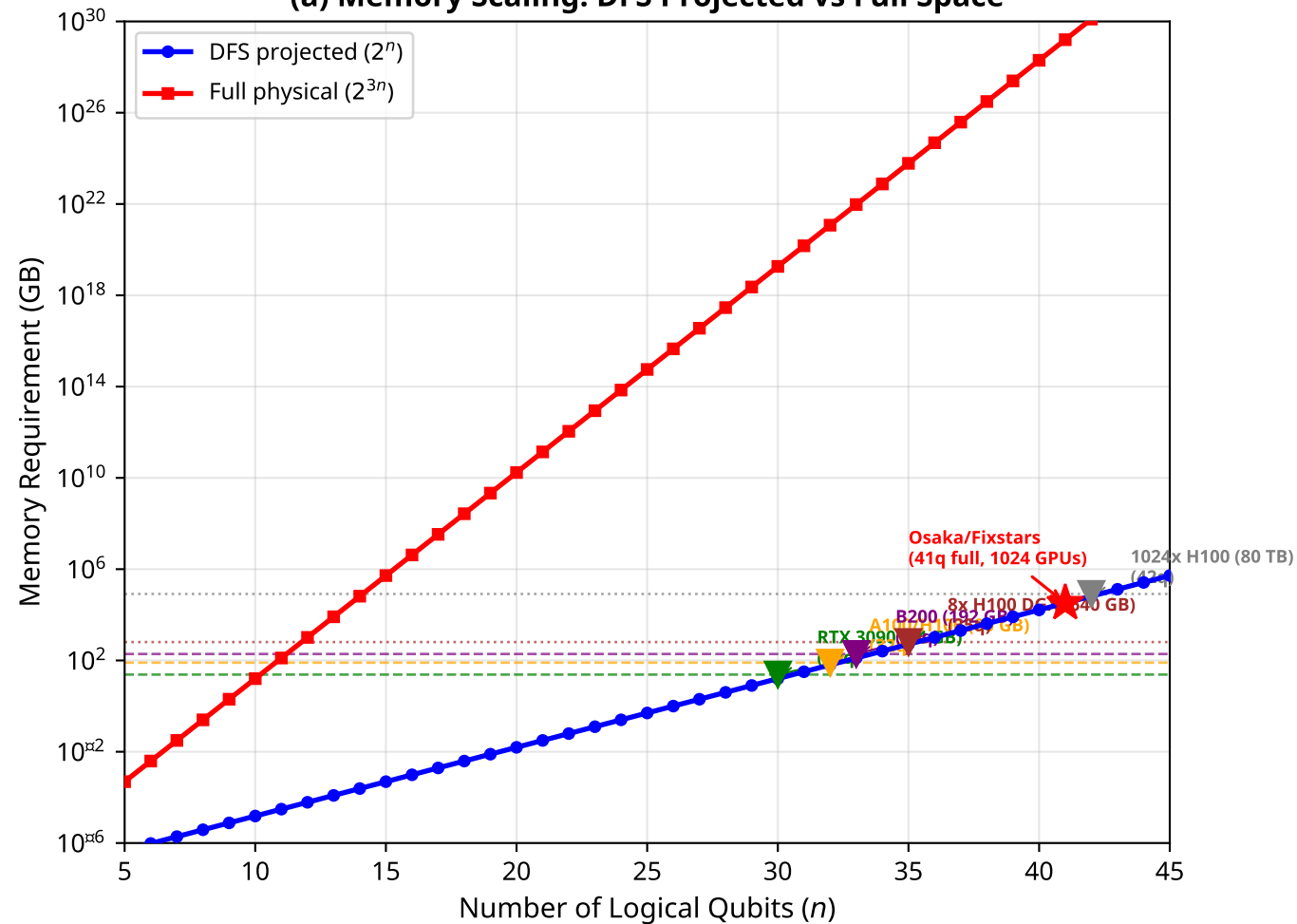
(a) Memory Scaling: DFS Projected vs Full Space
