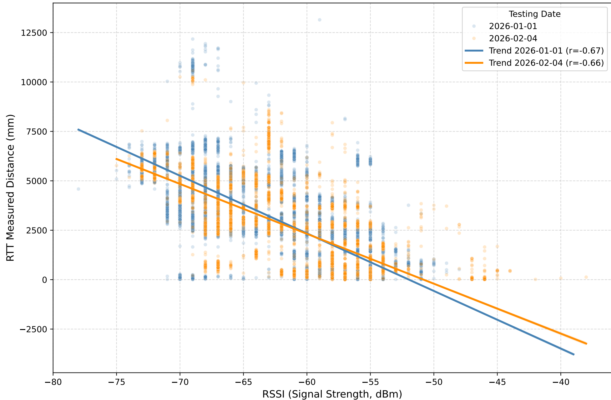
Global Time Drift: RSSI vs RTT (2026-01-01 vs 2026-02-04)
