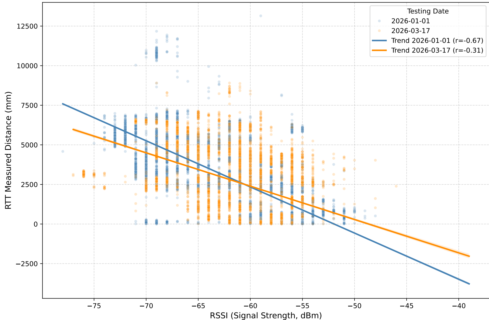
Global Time Drift: RSSI vs RTT (2026-01-01 vs 2026-03-17)
