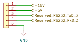
Reserved_RS232_602 Conn_01x05
