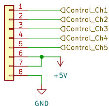
J602 Control_connector
