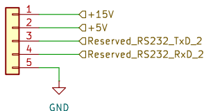
Reserved_RS232_601 Conn_01x05
