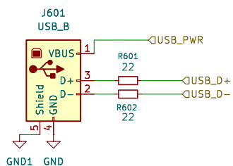
USB type B
