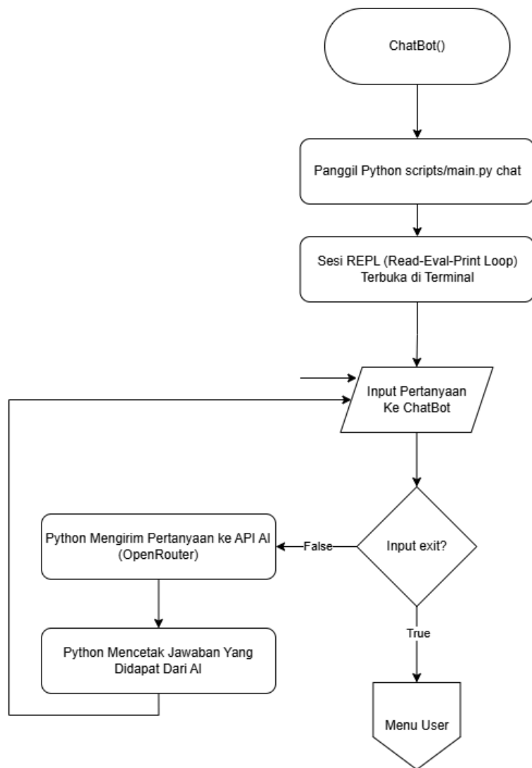
Gambar 2.11 Flowchart Fitur Chat AI Agent (user)
