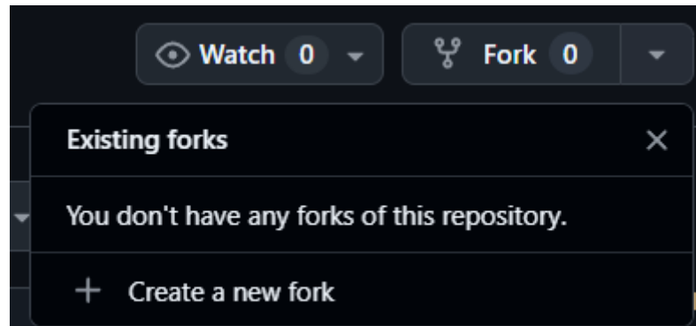
Gambar 6.1 Fork Repository
