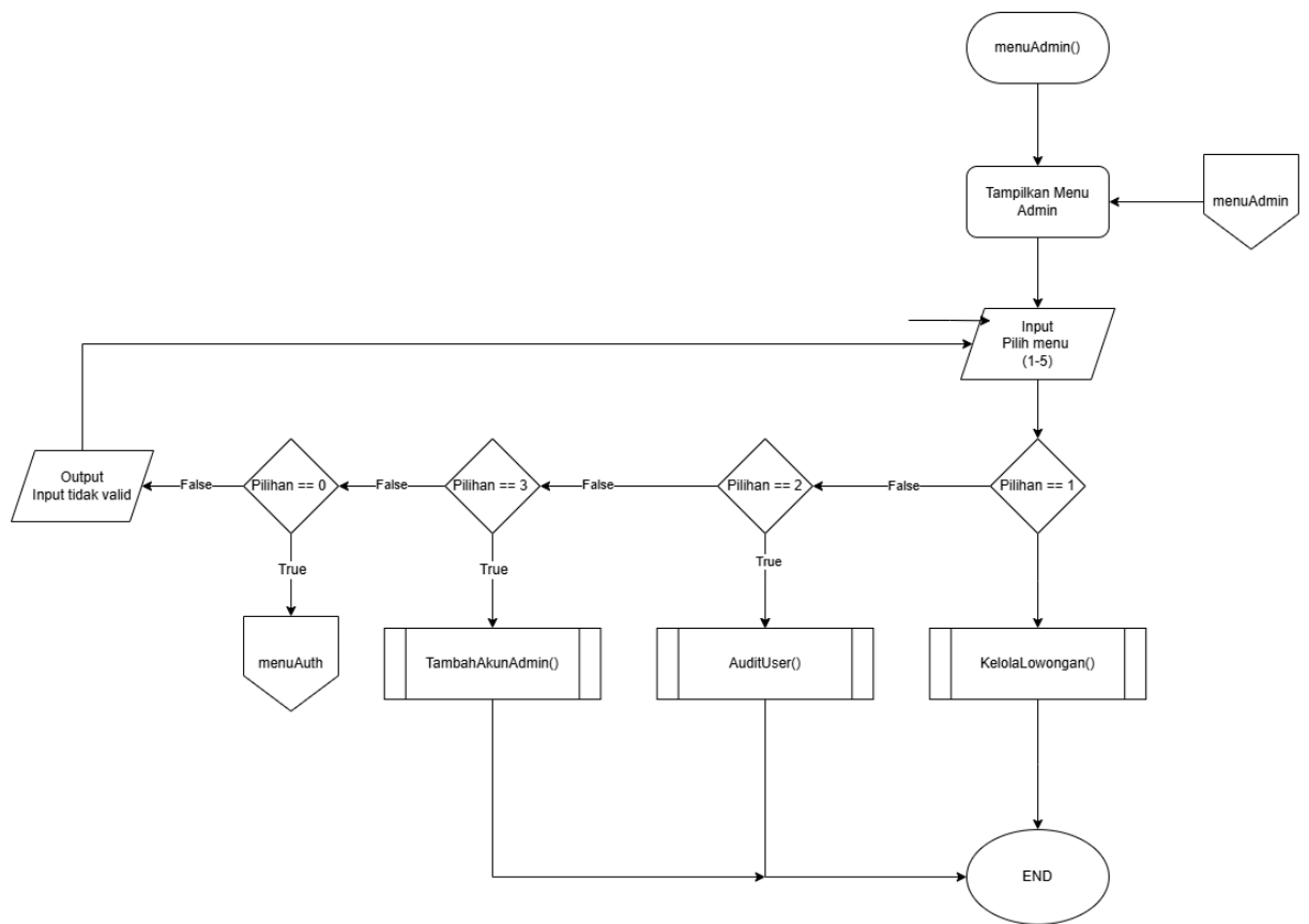
Gambar 2.2 Flowchart Menu Admin
