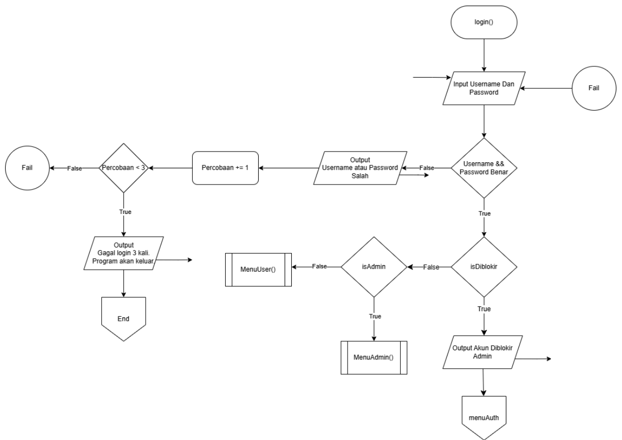
Gambar 2.4 Flowchart Fitur Login
