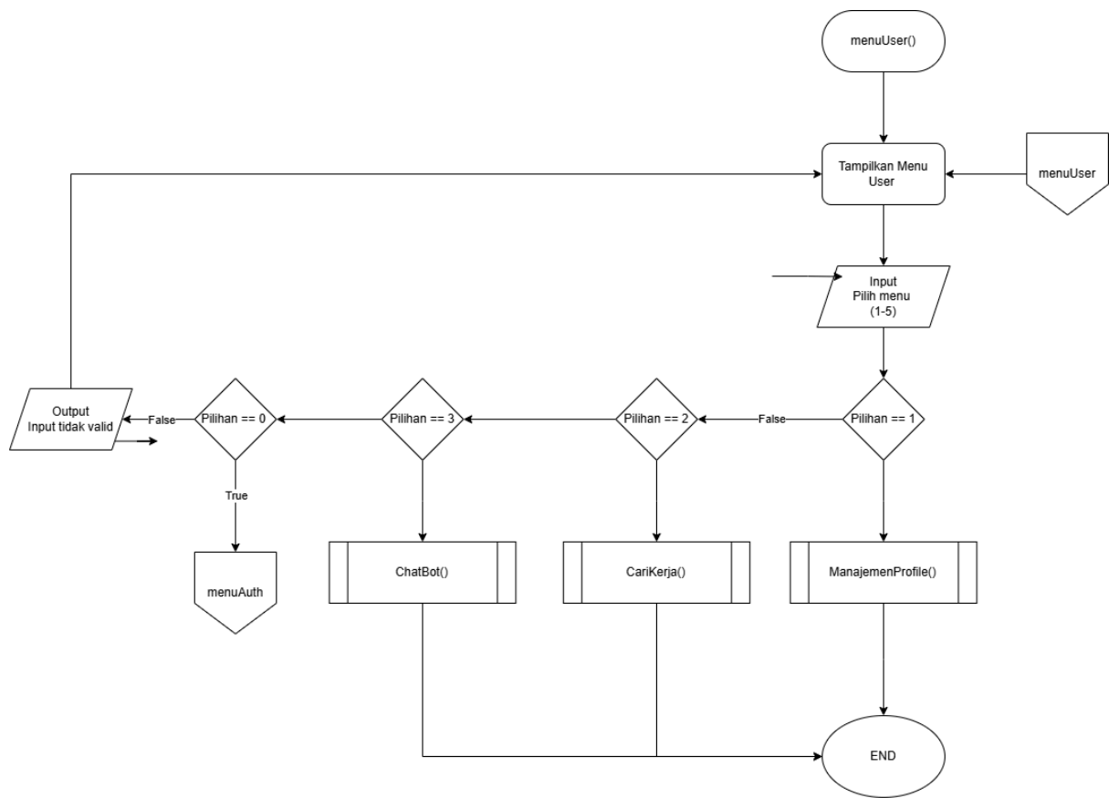
Gambar 2.3 Flowchart Menu User
