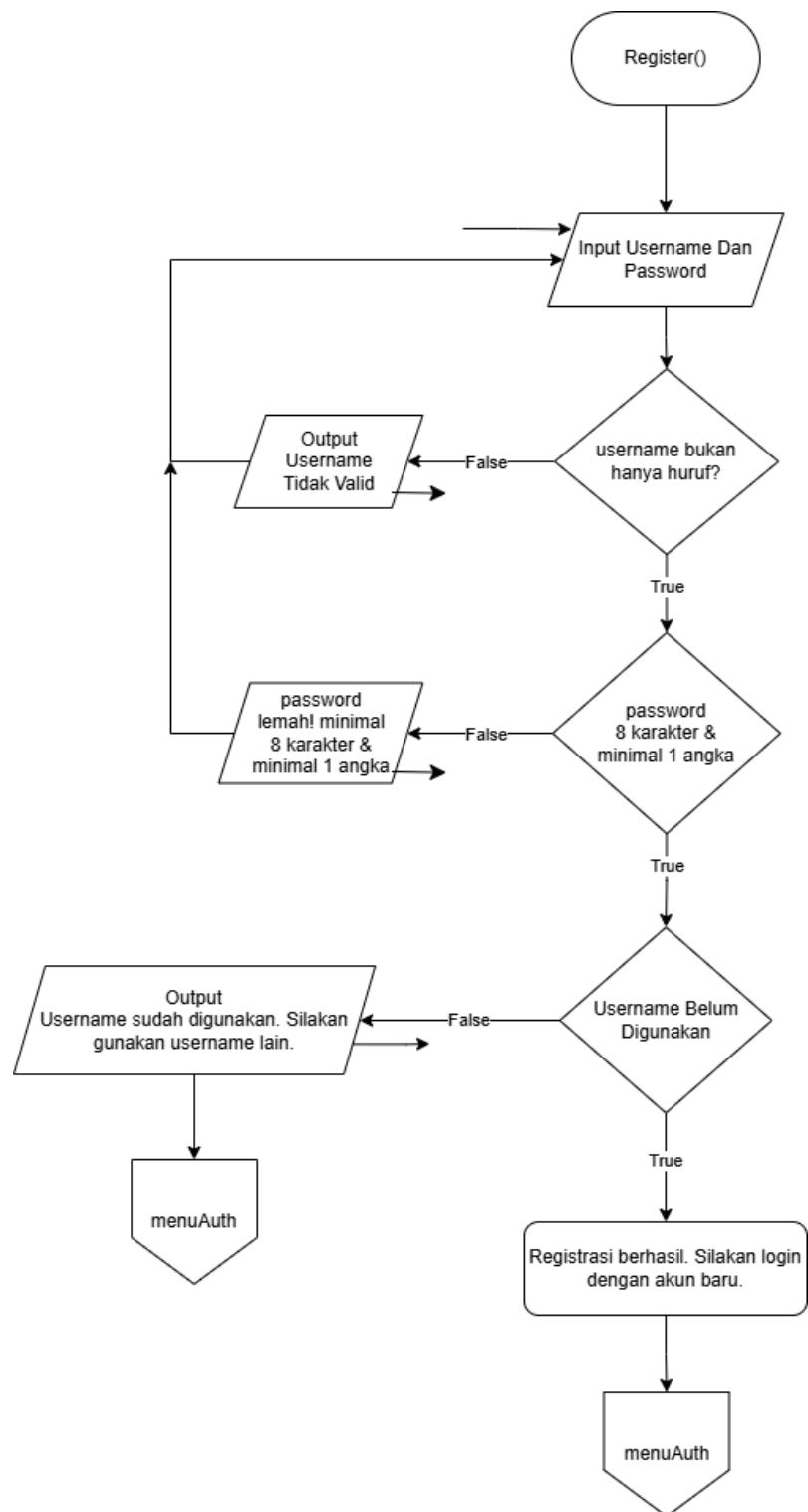
Gambar 2.5 Flowchart Fitur Register
