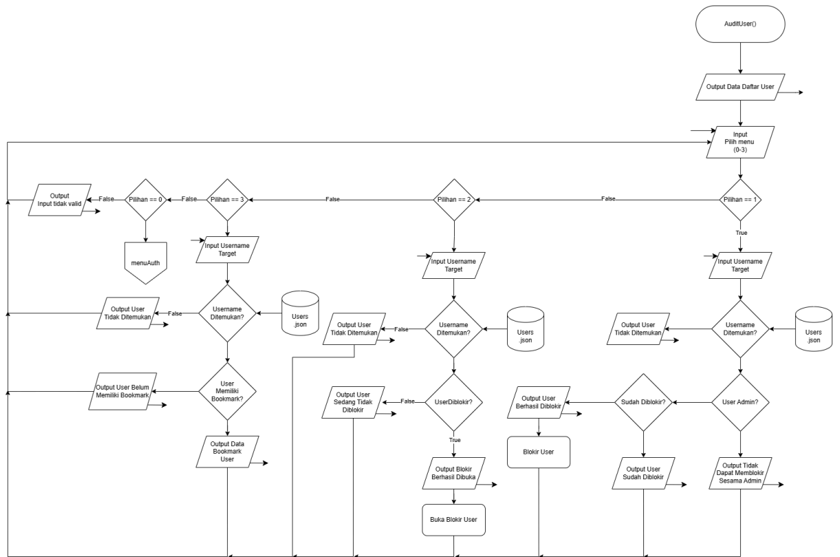
Gambar 2.7 Flowchart Menu Audit User (Admin)
