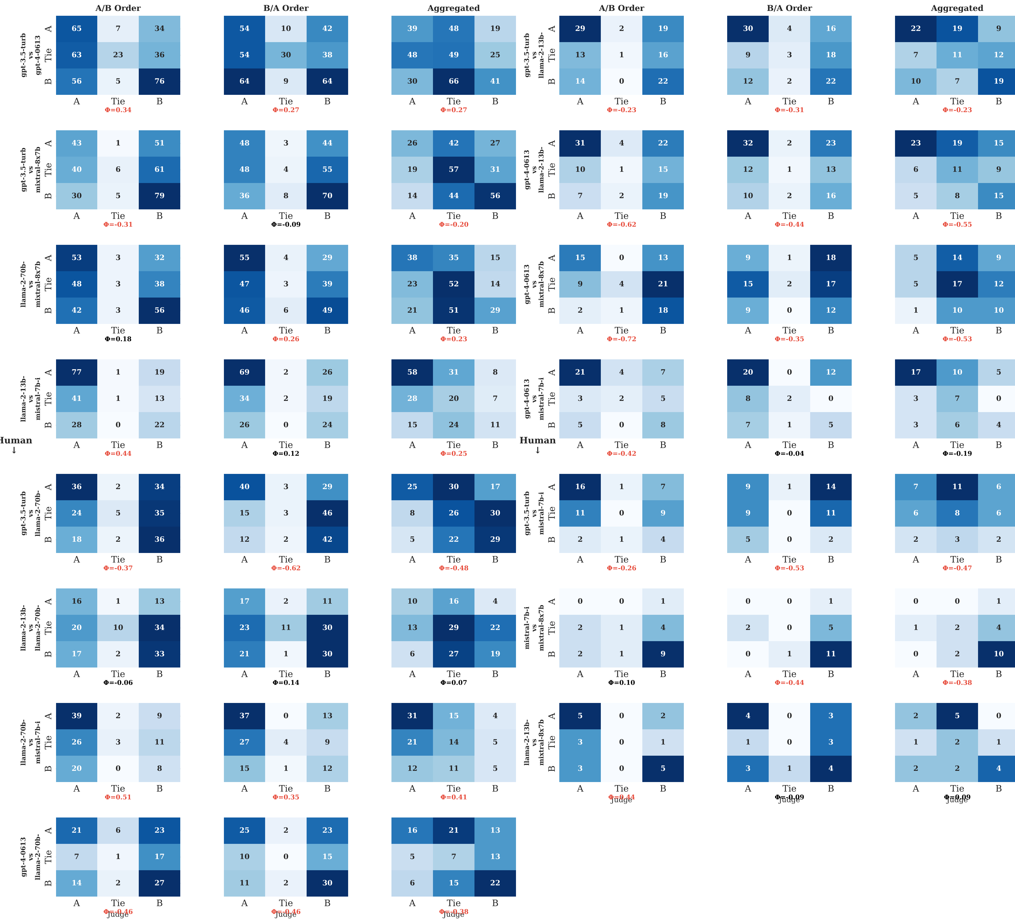
Confusion Matrices - gpt-3.5-turbo (OpenAI) Rows: Human verdict | Cols: Judge verdict | \Phi = FaviScore
