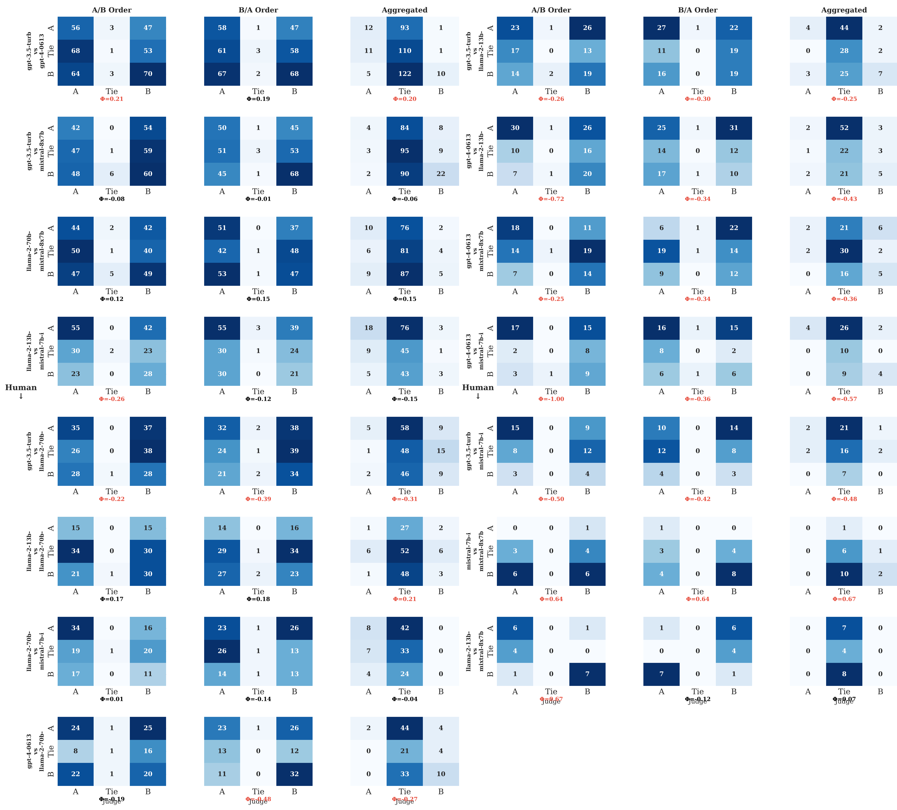
Confusion Matrices - llama2-70b (Meta) Rows: Human verdict | Cols: Judge verdict | \Phi = FaviScore
