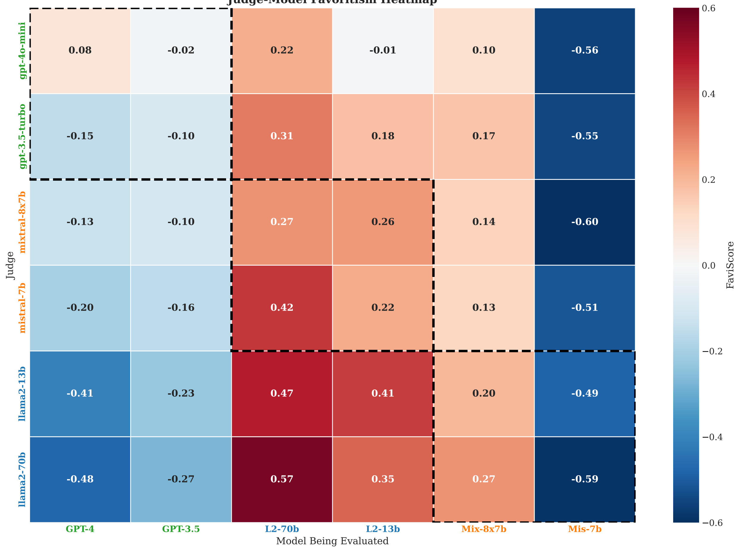
Judge-Model Favoritism Heatmap
