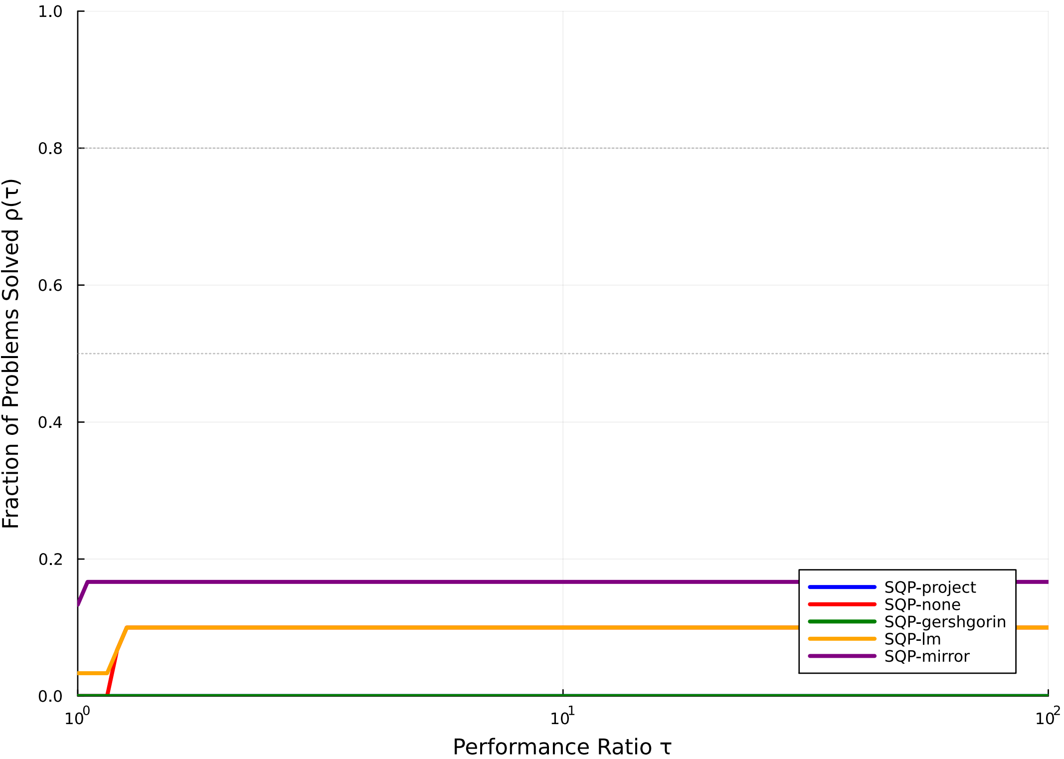
Performance Profile: hessian_convexification (Gesamtzeit)
