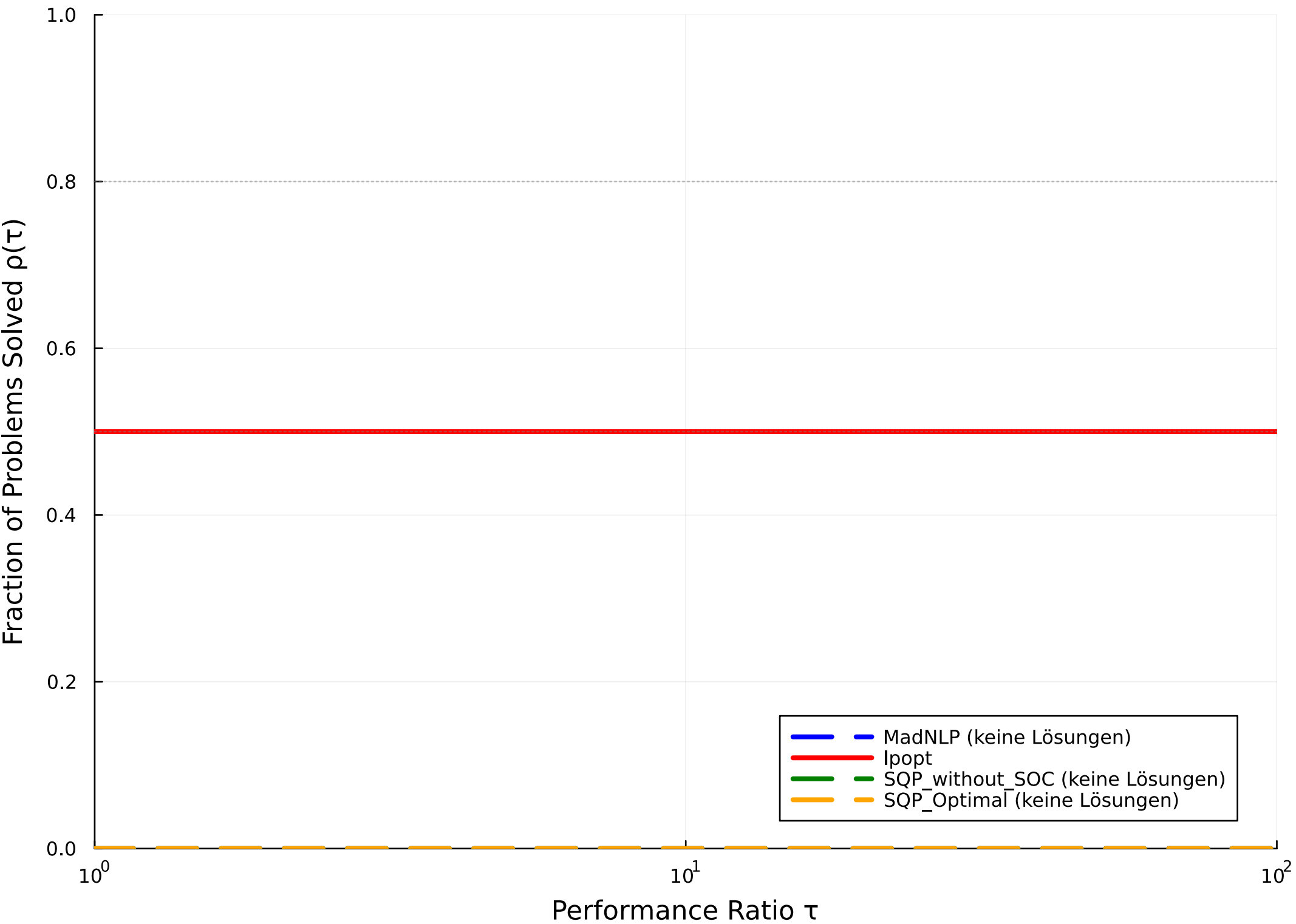
Performance Profile: large_benchmark_Large_Problems (Gesamtzeit)
