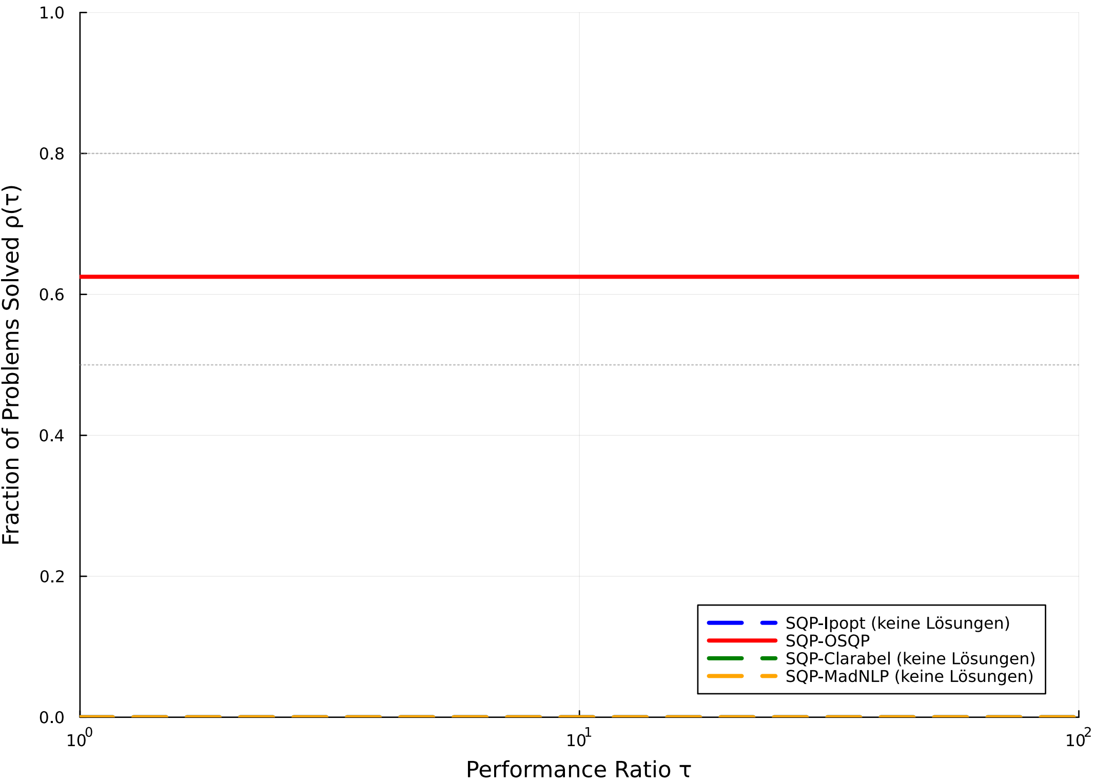
Performance Profile: qp_solvers_comparison (Gesamtzeit)
