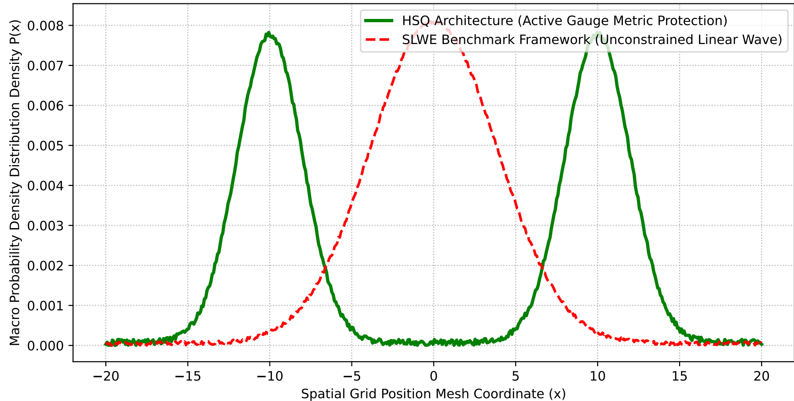
Quantum Random Walk Spatial Manifestation Profile (Phase Noise: 10.0%)
