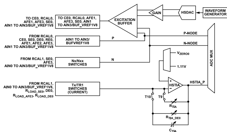
Figure 35. Switch Matrix High Level Diagram
