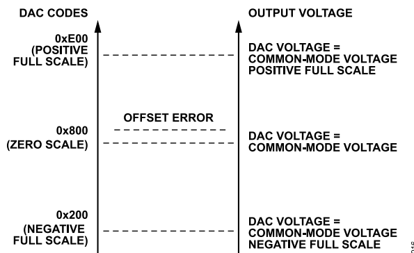
Figure 26. High Speed DAC Transfer Function
