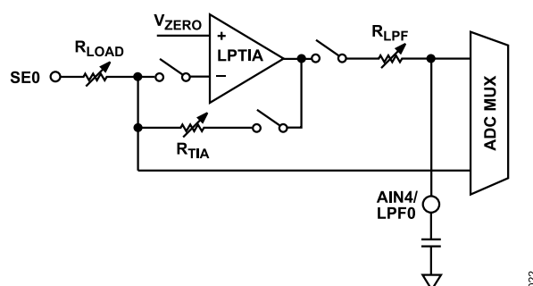
Figure 33. Low Power TIA Current Input Channel to the ADC
