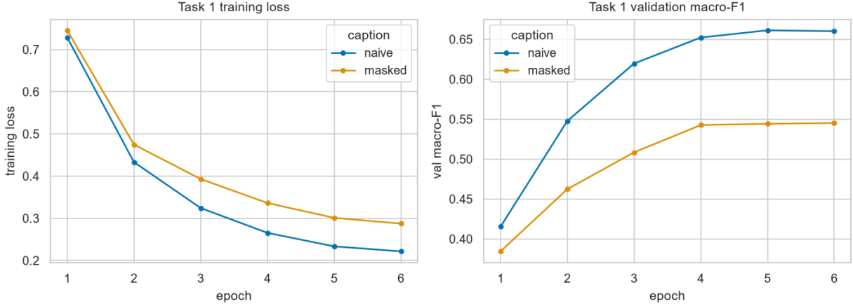
Figure 5: Task 1 learning curves, masked and naive conditions. The naive run tracks persistently higher on validation — the shortcut is visible during training, not only in the final metric.
