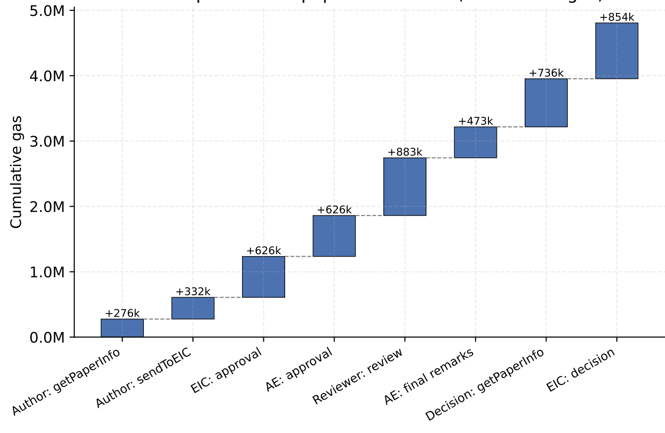
Gas to publish one paper end-to-end (total 4.81M gas)
