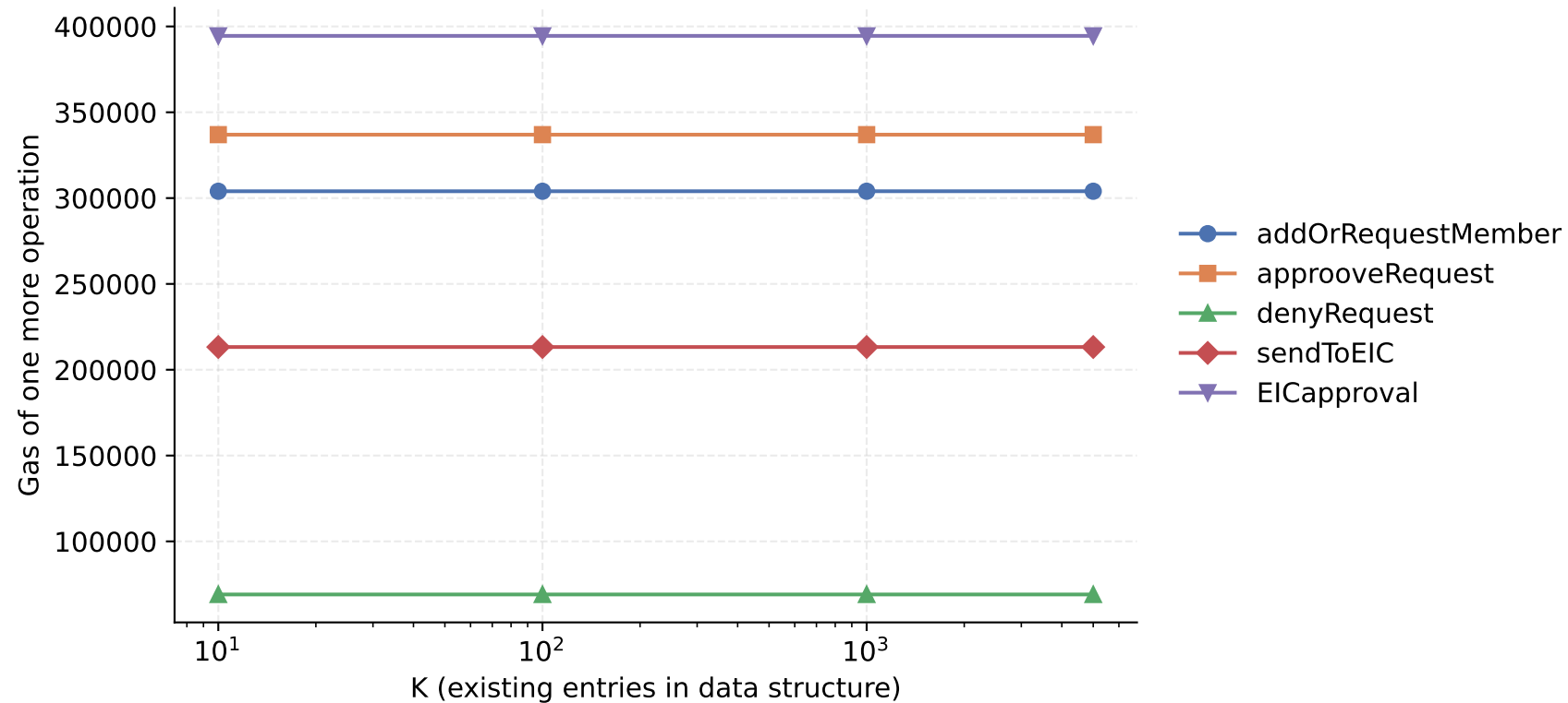
State-growth scalability (flat lines => O(1) per op)
