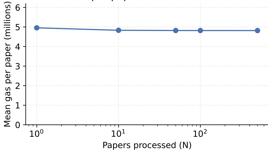
Cost per paper vs. workload size
