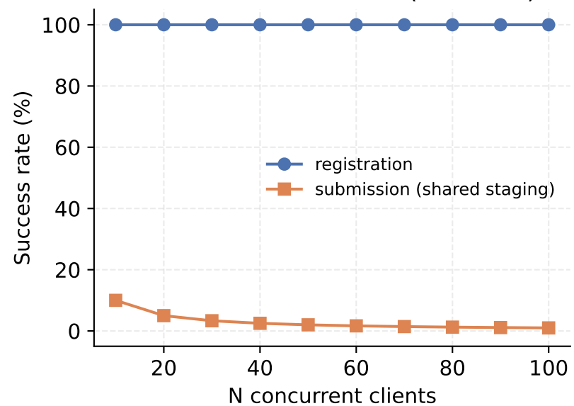
Success rate: shared staging serializes submissions (fails safe)
