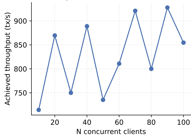
Registration throughput (parallel-safe workload)
