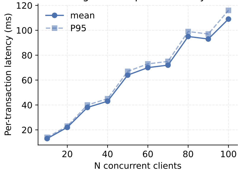
Registration per-tx latency
