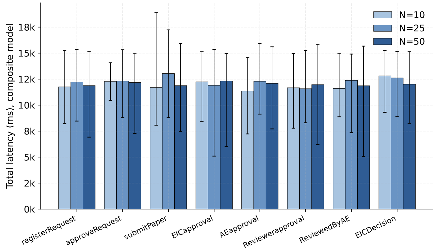
Composite total latency is stable across sample sizes (bars = mean, whiskers = min...P95; mainnet-sim model)
