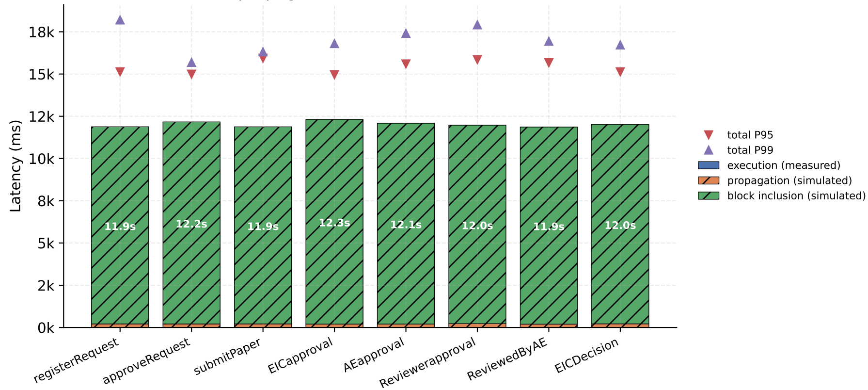
Confirmation-latency decomposition, N=50 samples/op (execution measured; propagation + inclusion from the mainnet-sim model)
