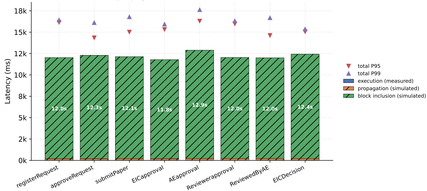
Confirmation-latency decomposition, 50 transactions/op (execution measured; propagation + inclusion from the mainnet-sim model)
