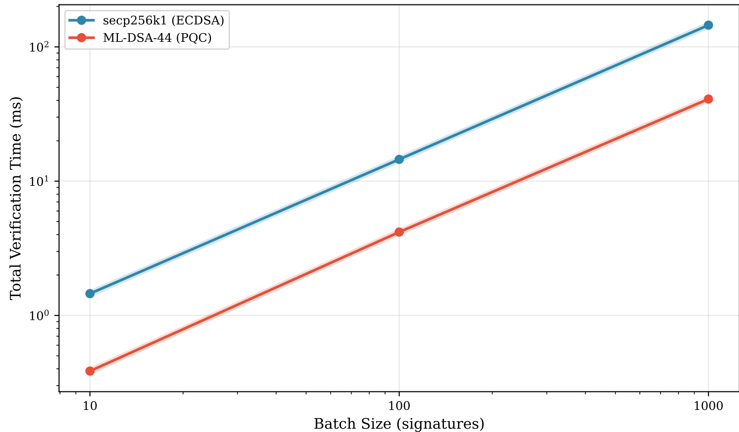
Batch Verification Performance
