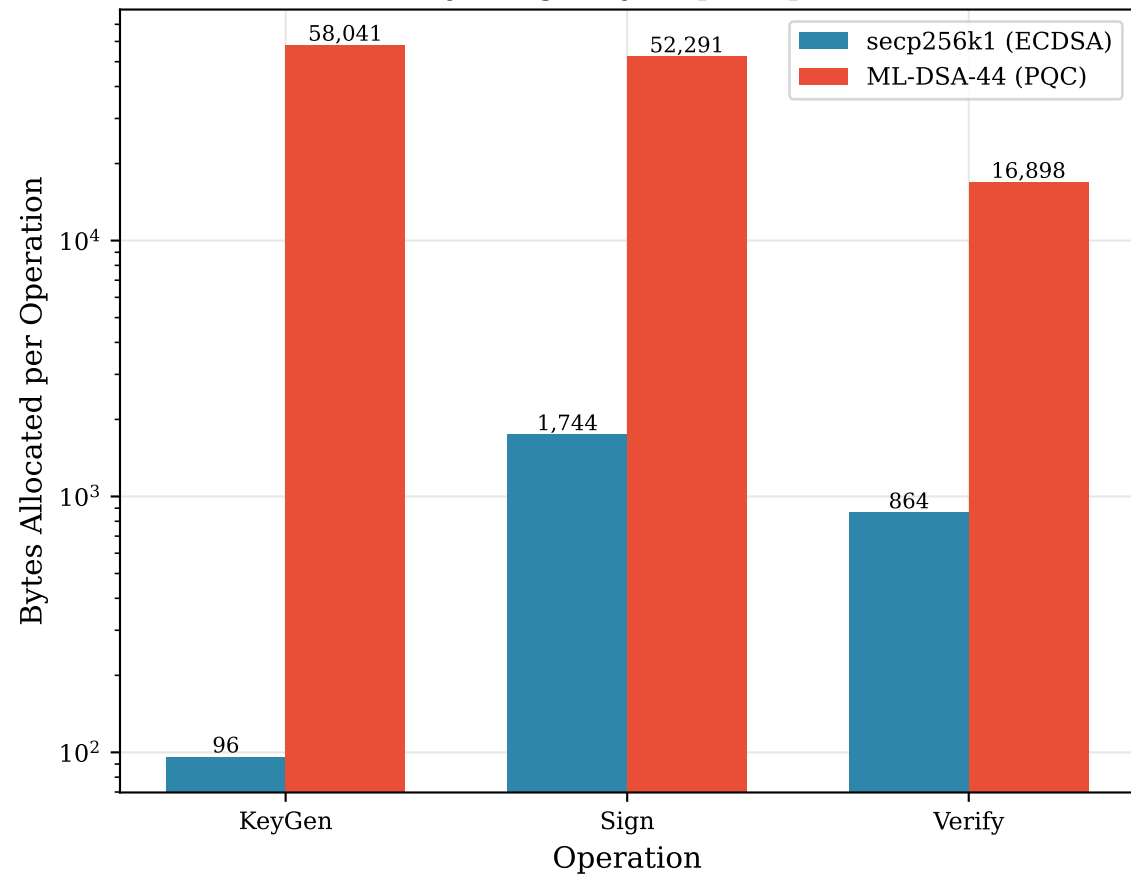
Memory Usage: Bytes per Operation
