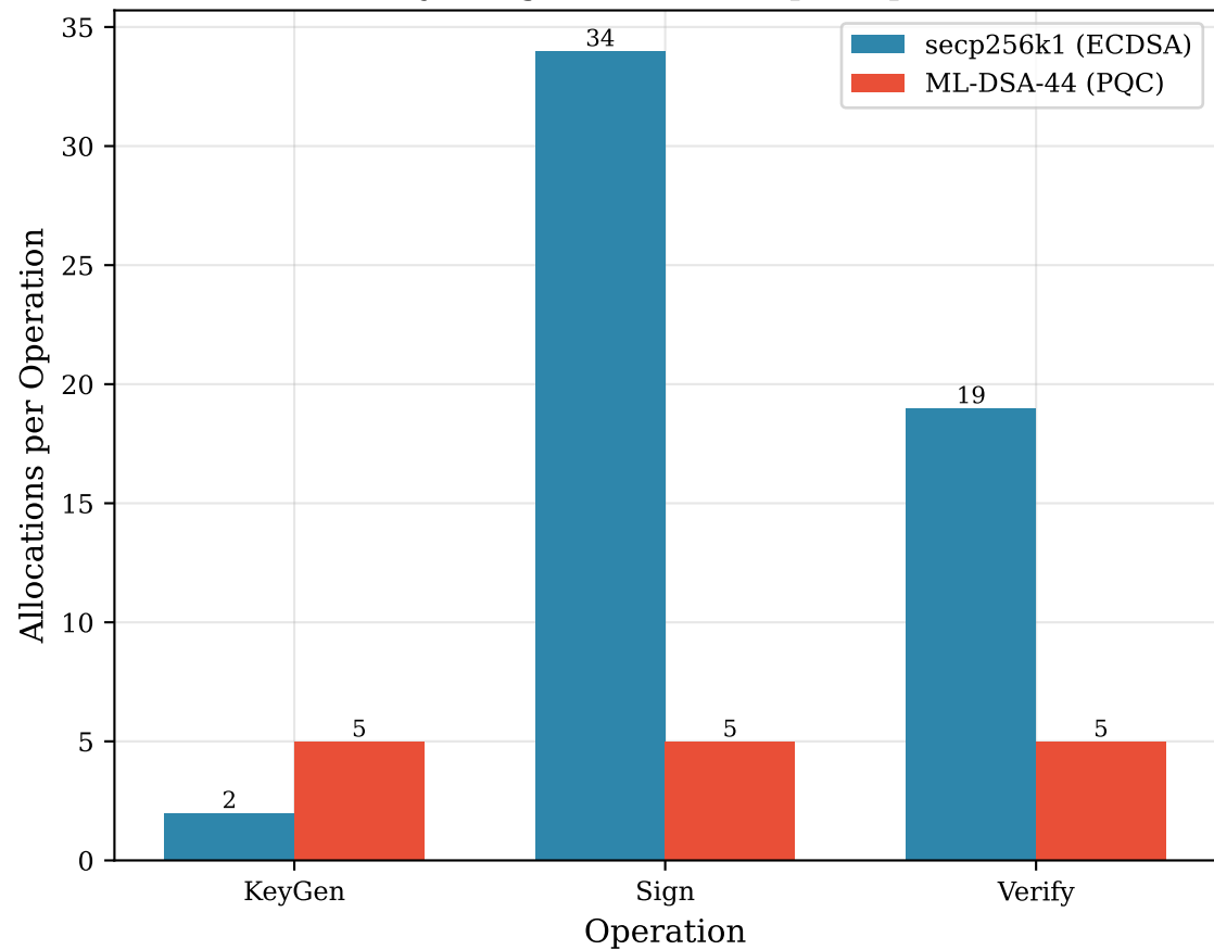
Memory Usage: Allocations per Operation
