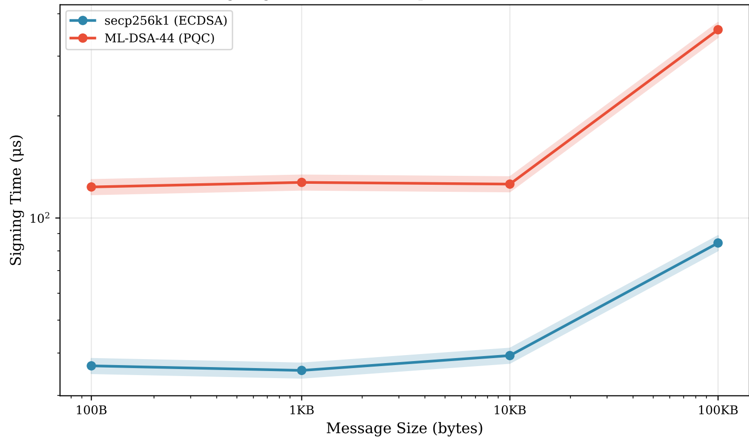
Signing Performance: secp256k1 vs ML-DSA-44
