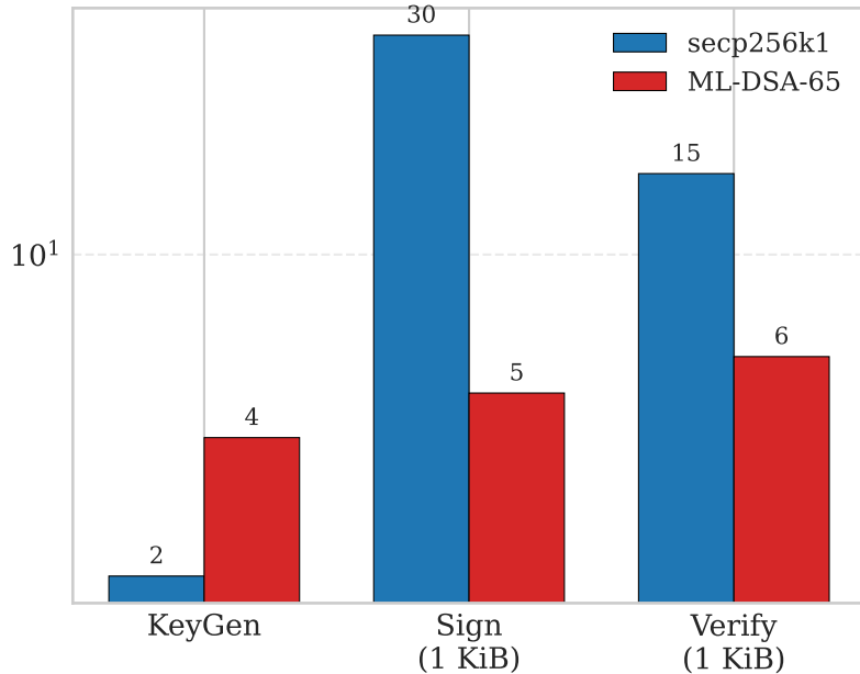
Allocations per operation (log)
