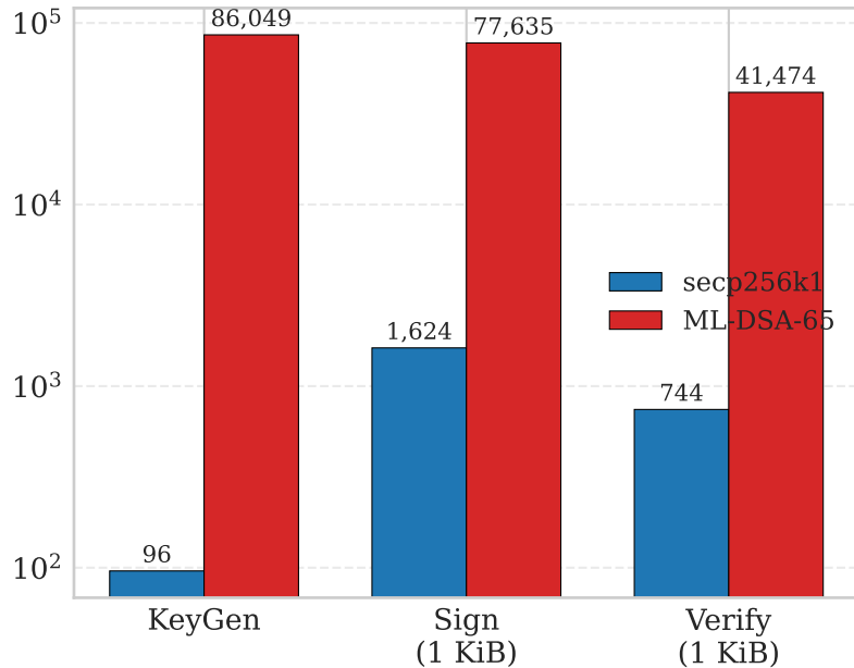
Bytes per operation (log)
