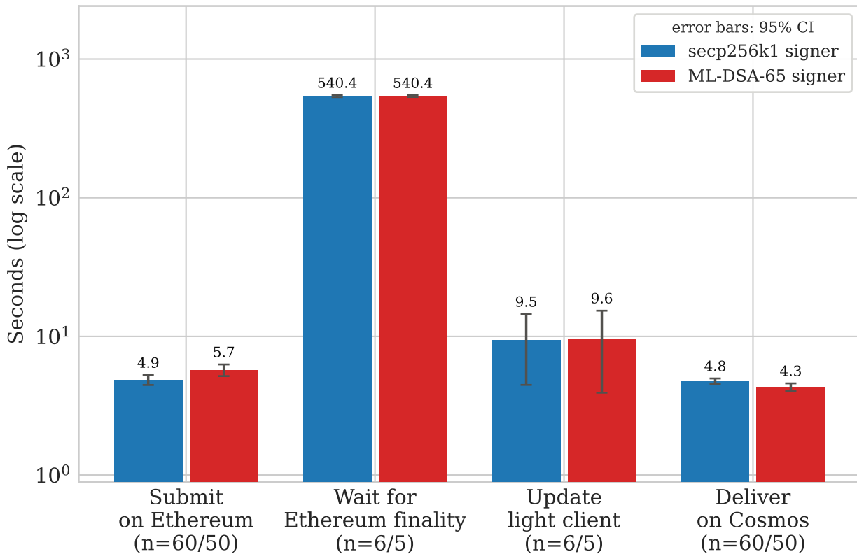
Time taken by each step of a migration (1 transfer)
