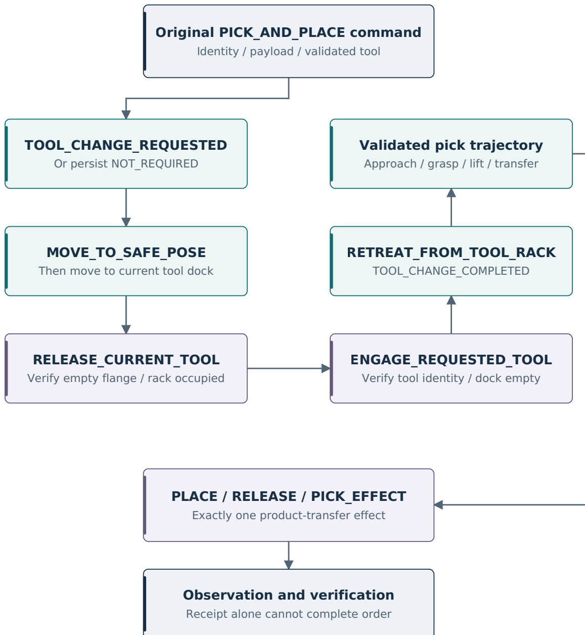
Figure 9. SIMULATOR DESIGN implemented execution sequence; final acceptance status is stated separately. A valid original PICK_AND_PLACE intent is durable before cell preparation. Selection and availability checks can reject before any transfer. If the active tool is correct, TOOL_CHANGE_NOT_REQUIRED is recorded and the preparation branch is bypassed. Otherwise dock, release/empty-flange, engagement/tool-ID and retreat events share the original command identity. Restart never treats a missing reply as permission for another pick.
