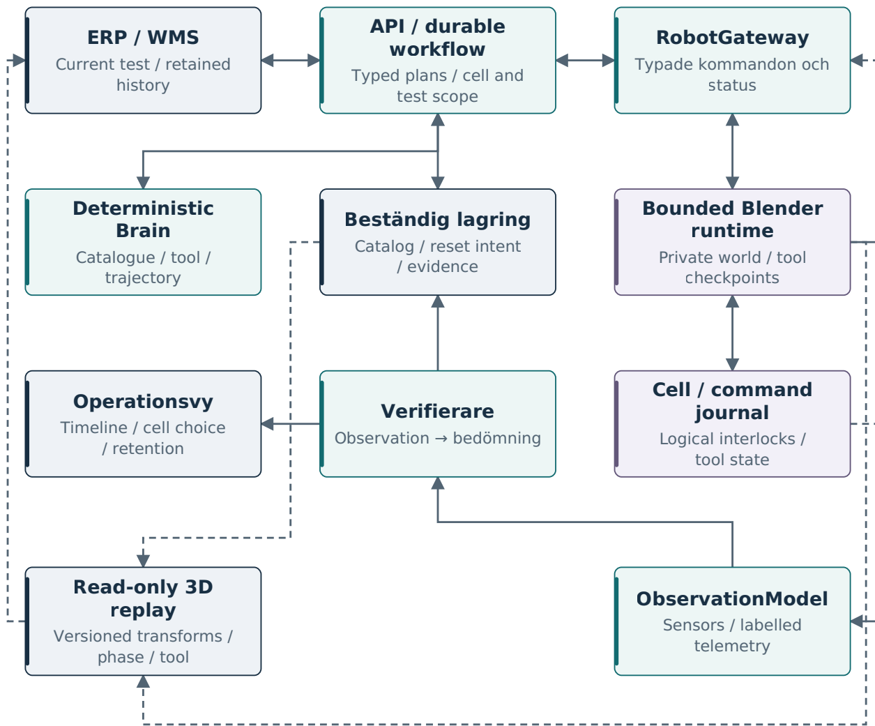
Figure 2. SIMULATOR_DESIGN architecture; revision-specific acceptance is stated separately. The durable workflow validates observed plans and preserves original command identity. The bounded Blender runtime owns private world/ tool state and controller checkpoints. ObservationModel alone converts world data into WorldObservation with explicit sensor and simulated telemetry provenance; Verifier has no direct world path. Tool preparation shares the product-transfer command and does not add a transfer effect. Replay reads versioned artifacts. The API cell registry initializes new tests; retained archives remain read-only. Confirmed deletion removes the test world and catalog entry after bounded cleanup; display numbers become reusable. Clear retains the same test identity/number/cell, replaces execution data with an empty scene and increments its revision before permitting new work. Only anonymous request digests remain after completed deletion. The UI drains its own pending replay and snapshot response bodies before confirmed management; controls and polling resume after final refresh. Backend response-lifetime and running-work guards remain enforced. Neither action dispatches a pick or assigns a verdict. Deleting the active test leaves no active world; explicitly clearing an archive activates only its restored world. Lost acknowledgement still requires original journal plus fresh sufficient observation, with no replacement pick. Investigation reads job-scoped persisted evidence independently of replay. Explicit re-observation alone invokes reconciliation; navigation and downloads do not mutate the world.
