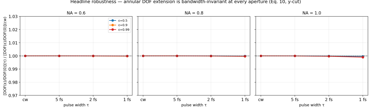
Figure 2: Robustness of the headline: the normalized DOF ratio [\text{DOF}(\varepsilon)/\text{DOF}(0)](\tau) relative to its cw value, for \varepsilon = 0.5, 0.9, 0.99 at \text{NA} = 0.6, 0.8, 1.0 .
