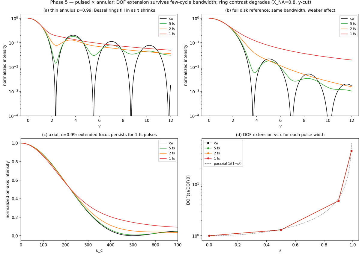
Figure 1: Pulsed annular focusing at NA = 0.8 : transverse ring filling vs. \tau at \epsilon = 0.99 ; full-disk reference; persistence of the extended axial focus at 1 fs; and the DOF ratio following the paraxial law for all \tau . [TODO: replace with publication-quality re-render]
