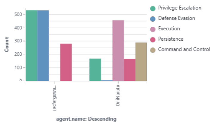
Top tactics by agent
