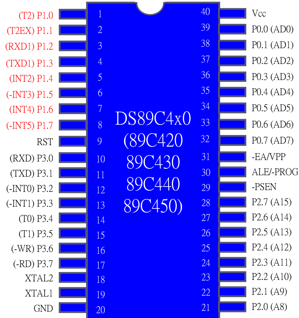
DS89C4x0 pin diagram
