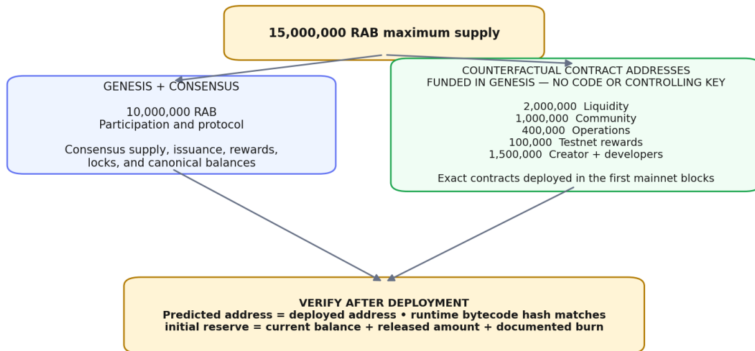
Figure 3. Genesis funds deterministic future contract addresses; verified contracts are then deployed at those exact addresses in the first mainnet blocks.
