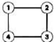
CONNECTED
