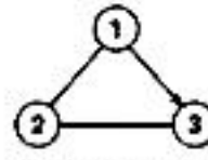
CYCLIC
