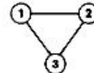
UNWEIGHTED
