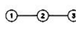
ACYCLIC
