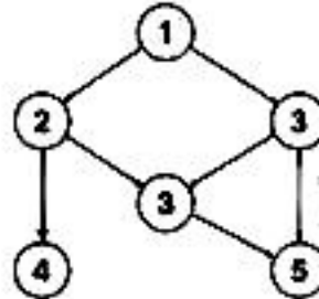
GENERAL GRAPH
