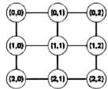
GRID (2D)
