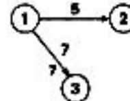
WEIGHTED
