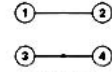
DISCONNECTED
