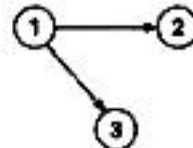
DIRECTED
