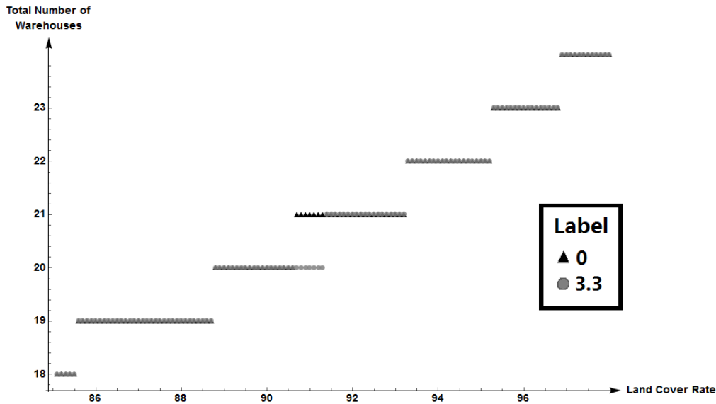
Figure 8: Relations between warehouses Land Cover Rate with/without \eta
