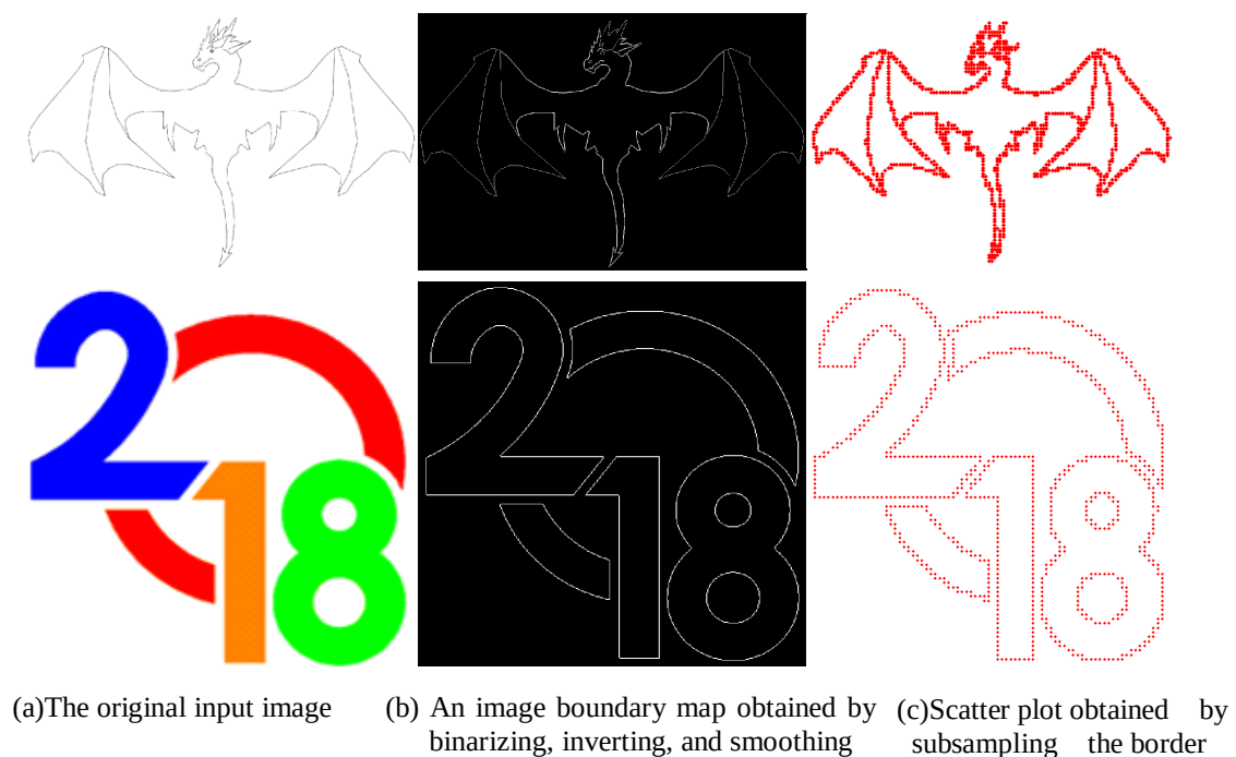
Fig 2. Effect of image preprocessing
