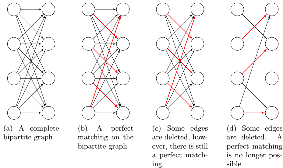
Figure 3.5: Examples of matching. Edges in the matching are highlighted red
