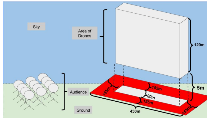
Figure 5.2: Clearance area for the drone display
