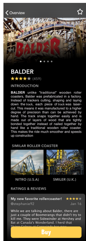
Fig. 13 Recommended system
