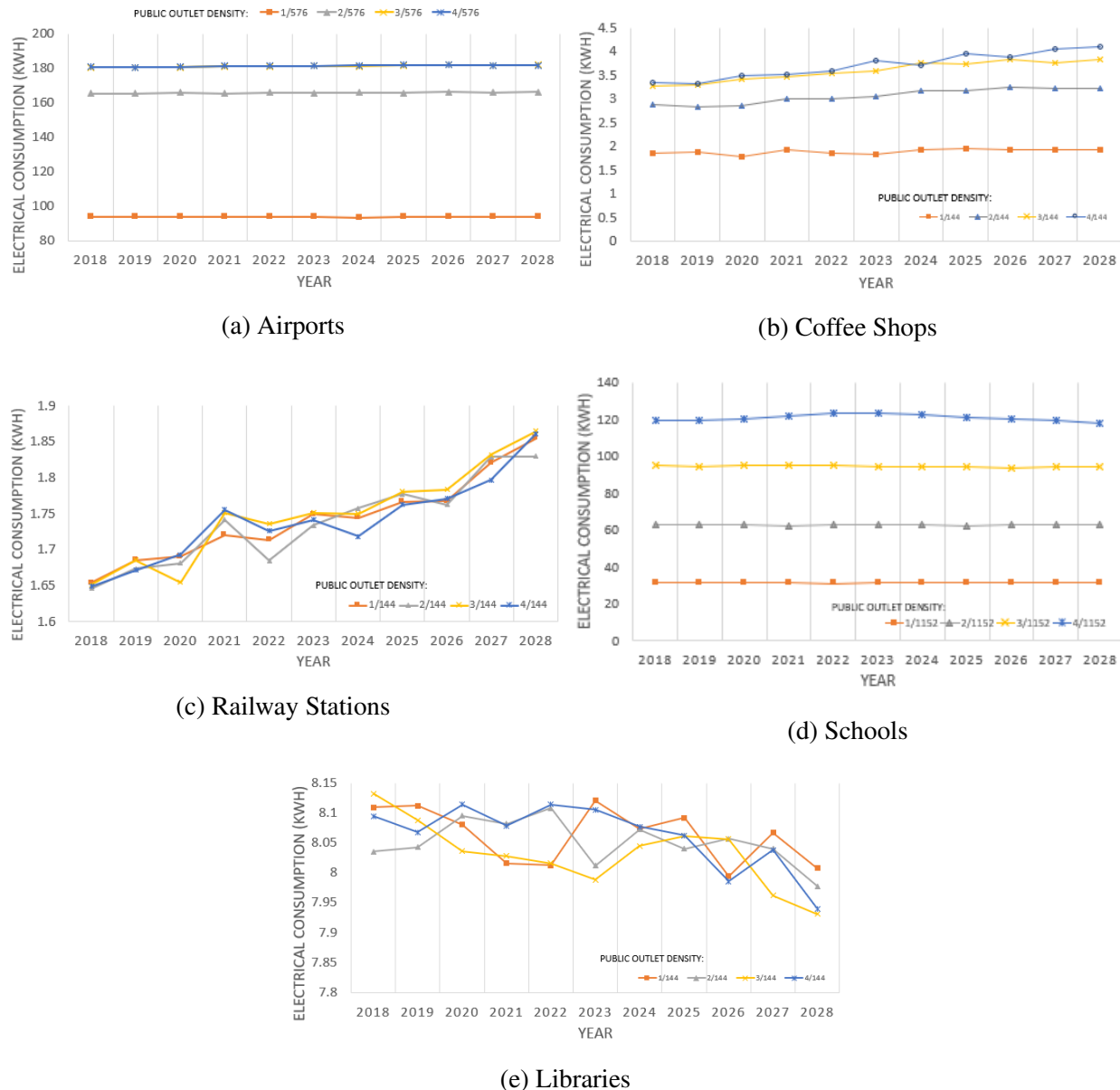
Figure 4: The forecasted daily electrical consumption (kWh) from 2018-2028 for different public outlet densities (colors) for each defined destination (a-e).
