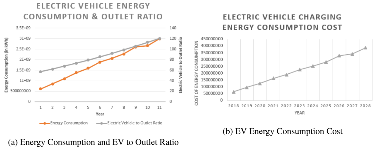
Figure 7: The projected energy consumption, electric vehicle to outlet ratio, and cost for electric vehicles for the next 10 years.
