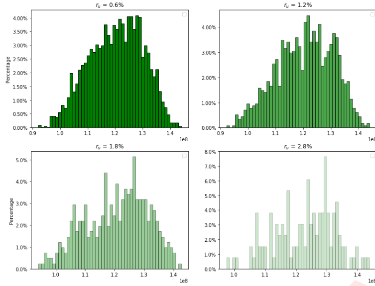
r_u Influence on Distribution of C_{total}^a \cdot dev of Eligible Stochastic Funding Plans
