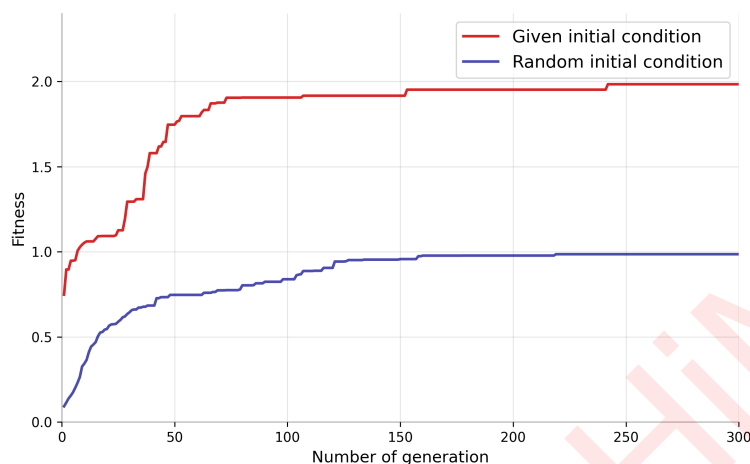
Figure 12: Convergence plot
