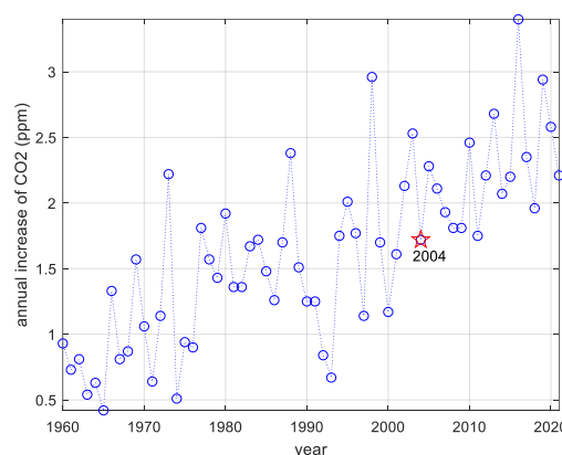
Figure 4.2 Annual increase of \text{CO}_2
