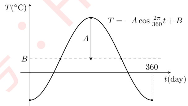
Fig. 1 Temperature curve
