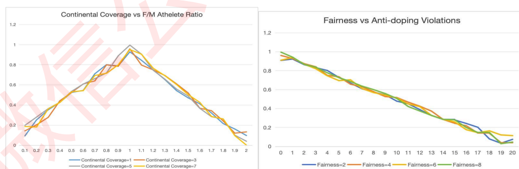
Figure 7: Multi-Factor Sensitivity Analysis
