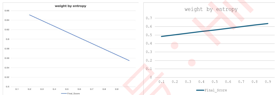
Figure 9: Method-Weight Sensitivity Analysis
