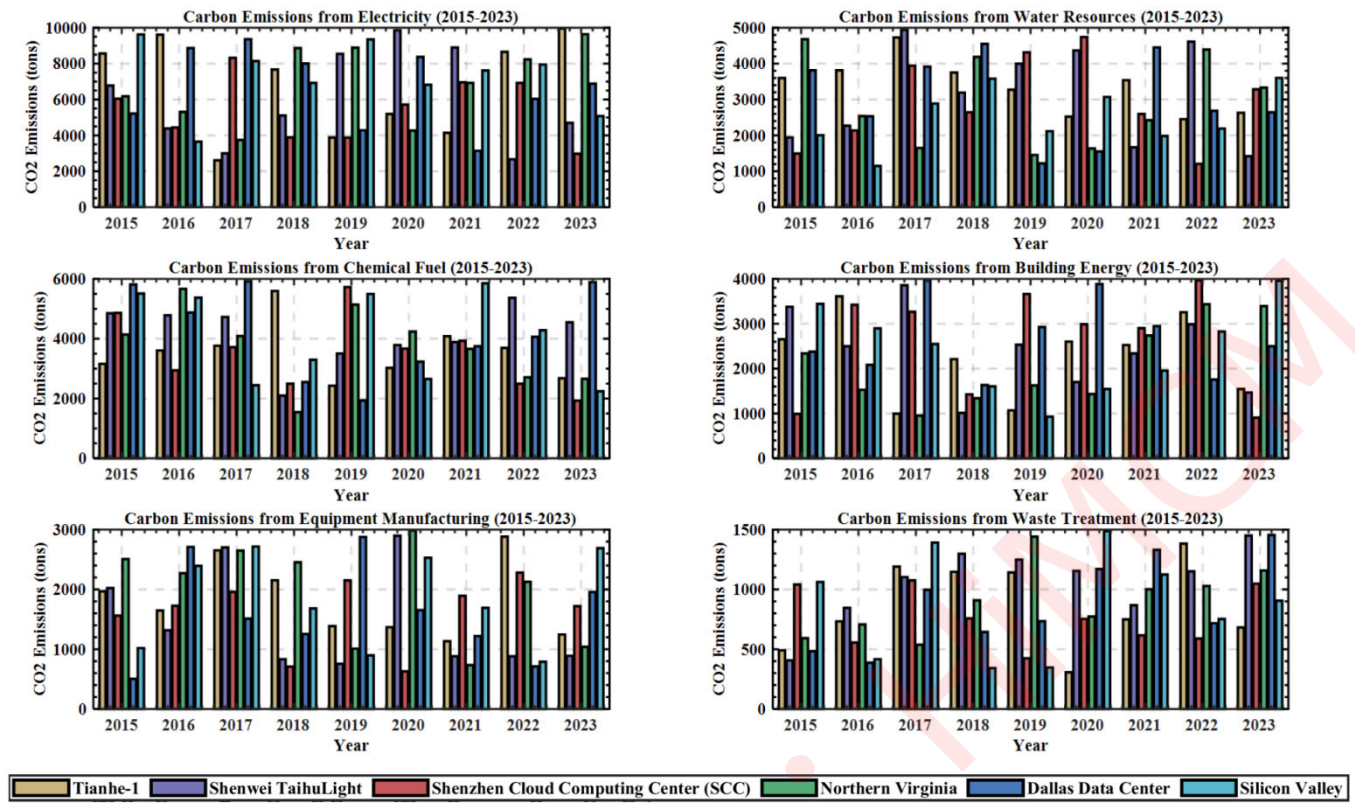
Figure. 6 Carbon Emission Measurement Results of the Six HPC Systems from 2015 to 2023
