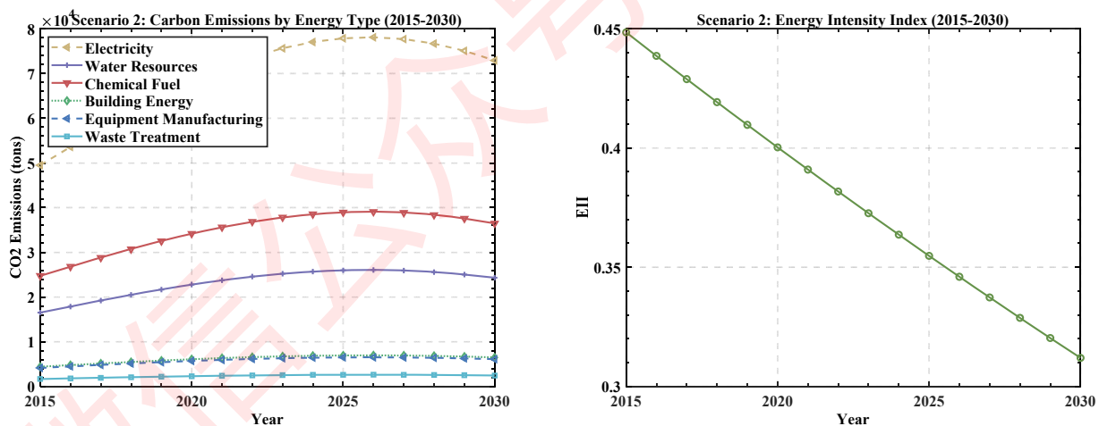
Figure. 9 Scenario 2 Simulation Results
