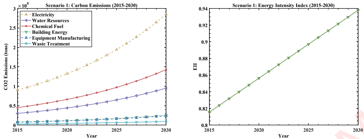
Figure. 8 Scenario 1 Simulation Results
