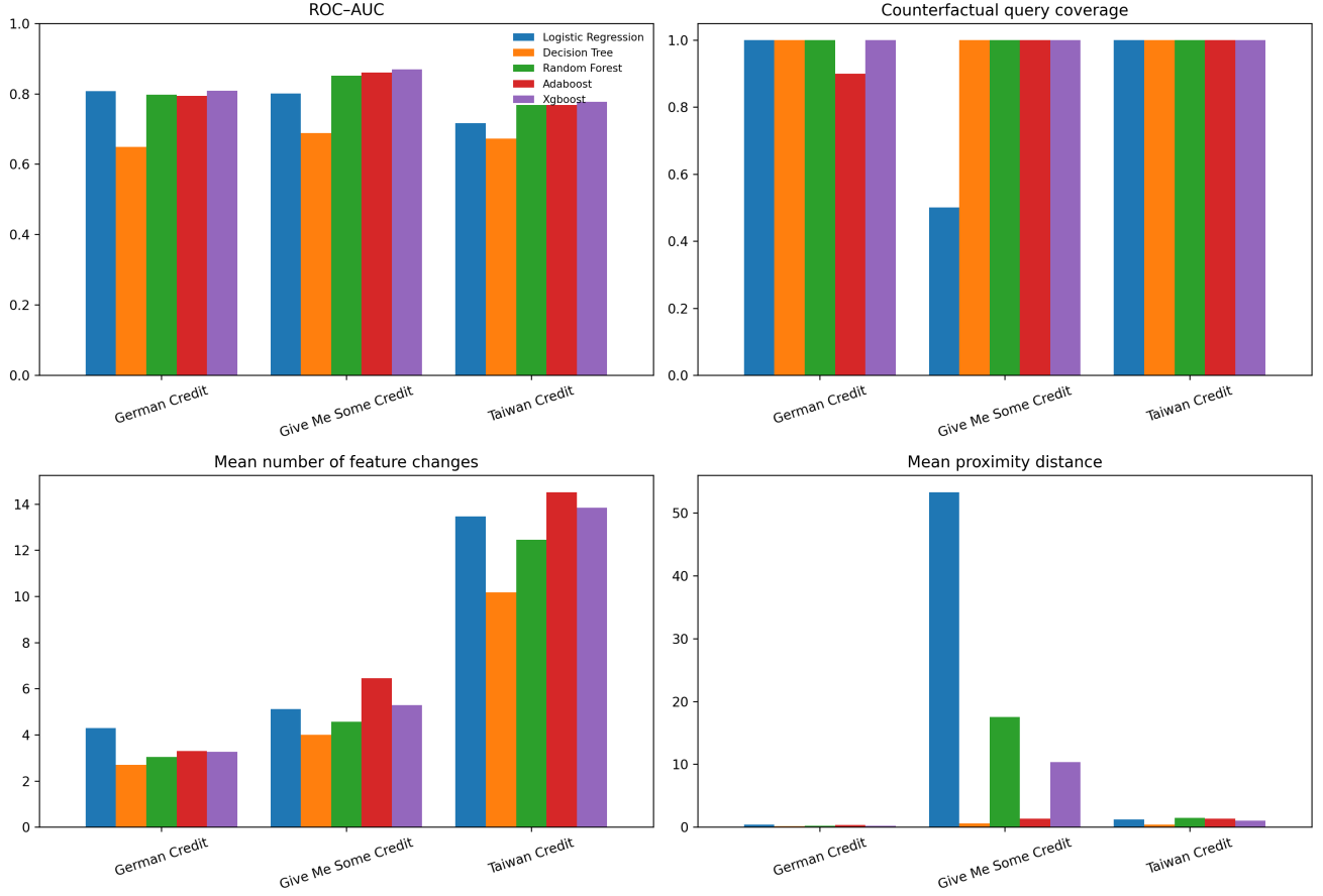
Predictive performance and DiCE recourse across model families
