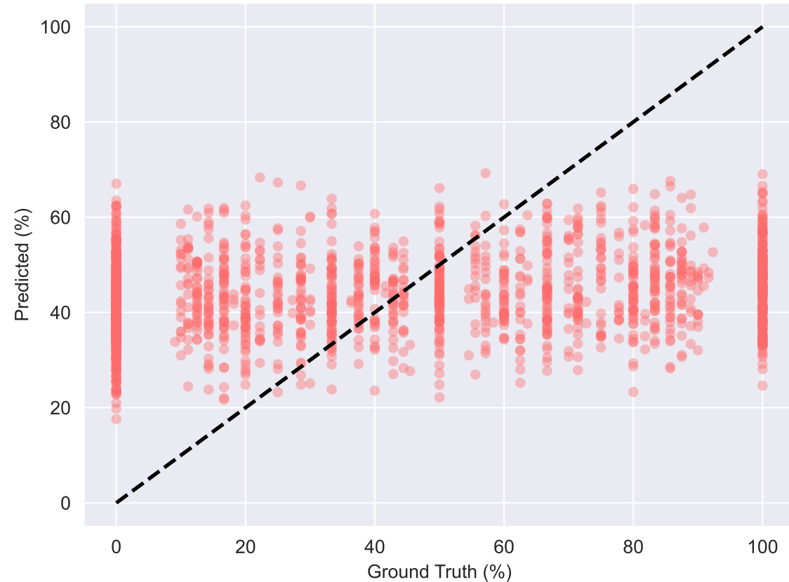
Baseline A RMSE: 35.33, NCC: 0.209
