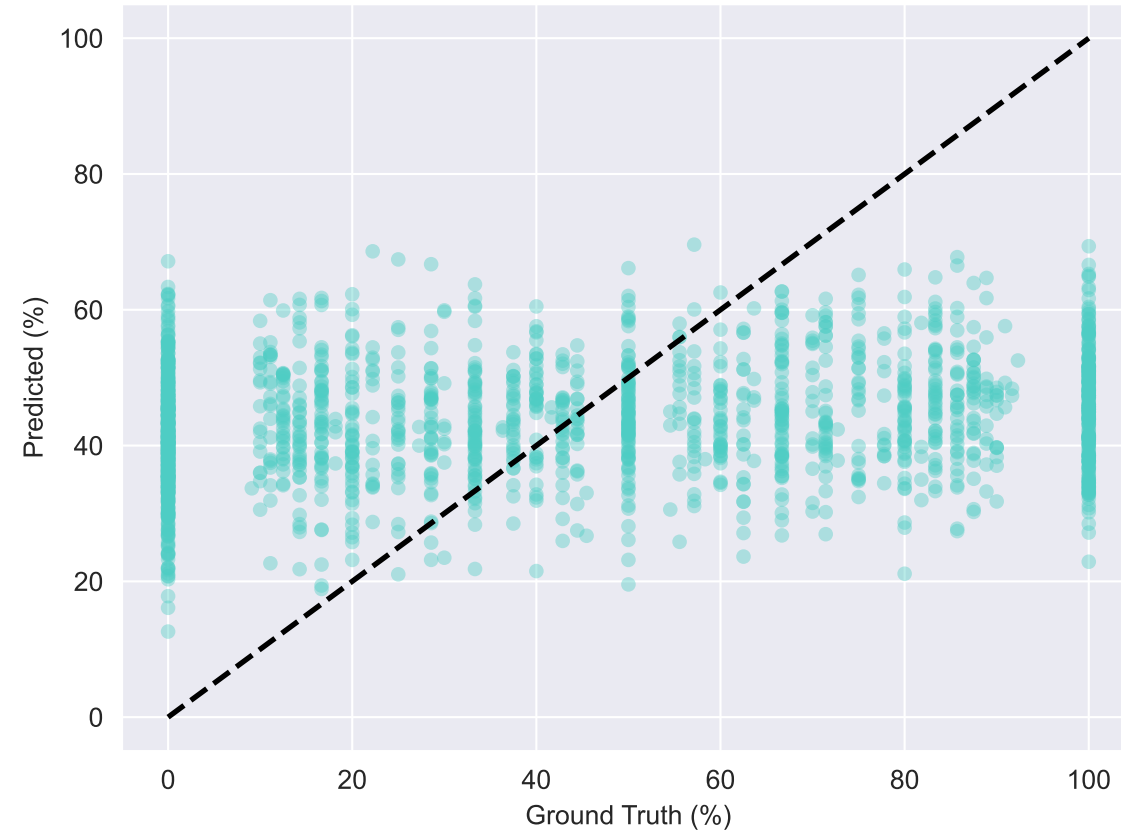
Baseline B RMSE: 35.33, NCC: 0.210
