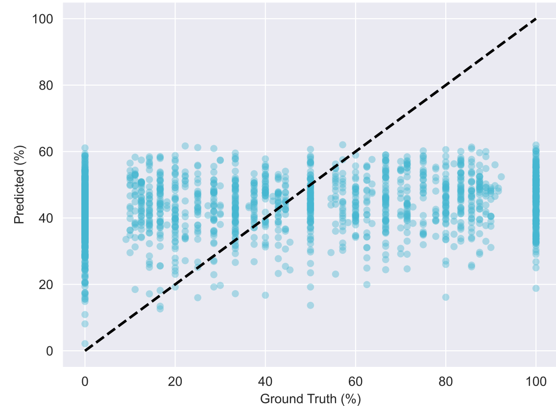
Baseline C RMSE: 35.34, NCC: 0.209
